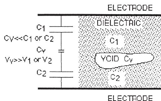
Figure 1. Void Between Electrodes
