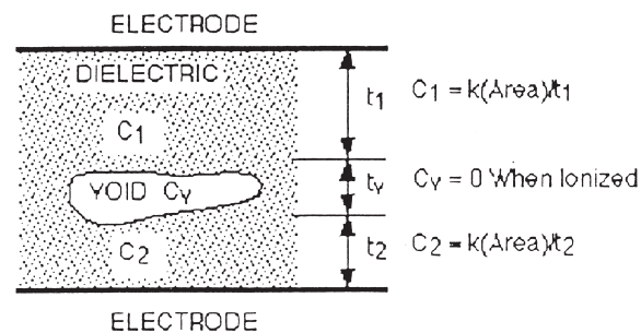
Figure 2. Equivalent Capacitors at Ionized Void
