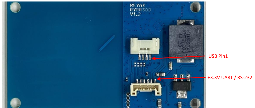
USB Interface Connector CVILUX CI4604M1HR0-NH
